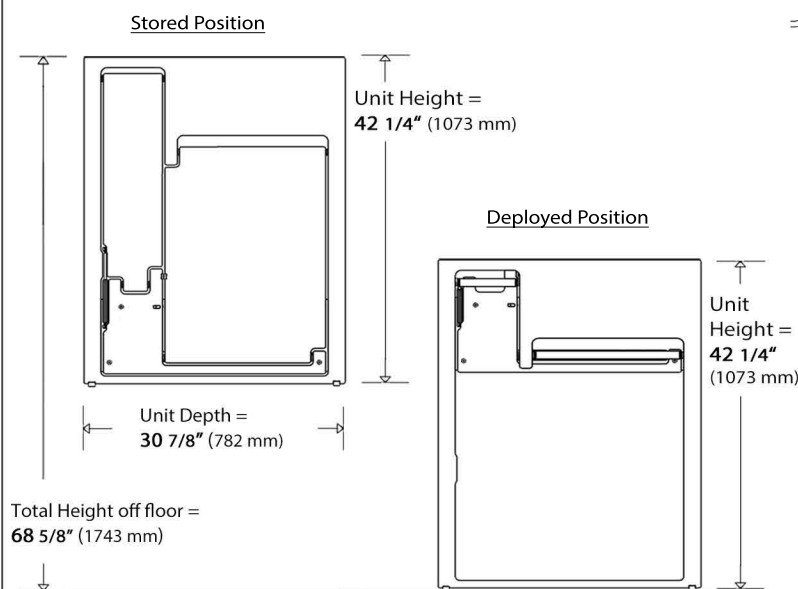
FRONT VIEW - Deployed and Stored Positions
