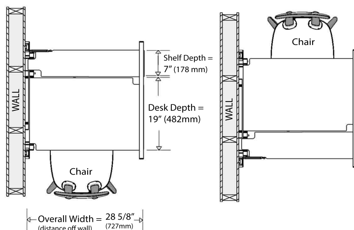
TOP VIEW - Deployed - Shown mounted on wall in either direction
