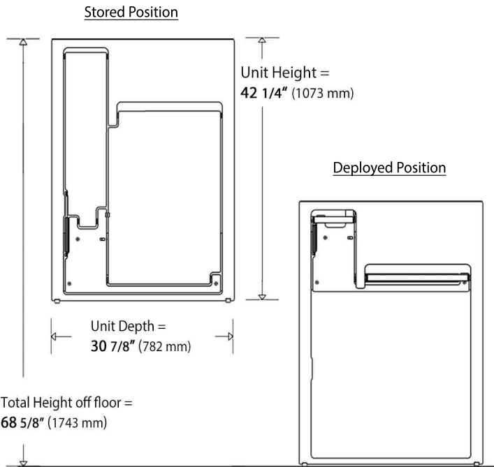
FRONT VIEW - Deployed and Stored Positions
