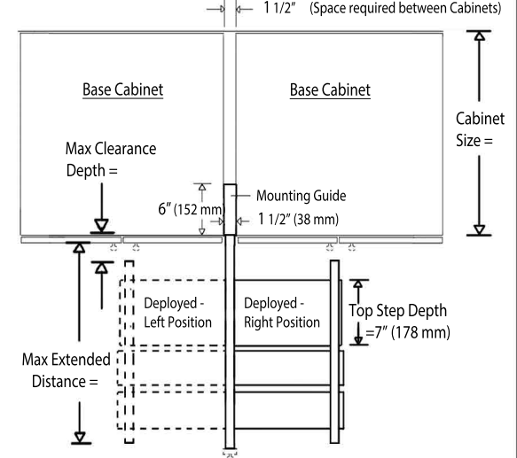
TOP VIEW - Mounted Between two X-Large Base Cabinets
