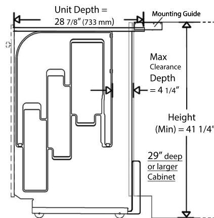
SIDE VIEW - Extended Closed Position (29" Model)
