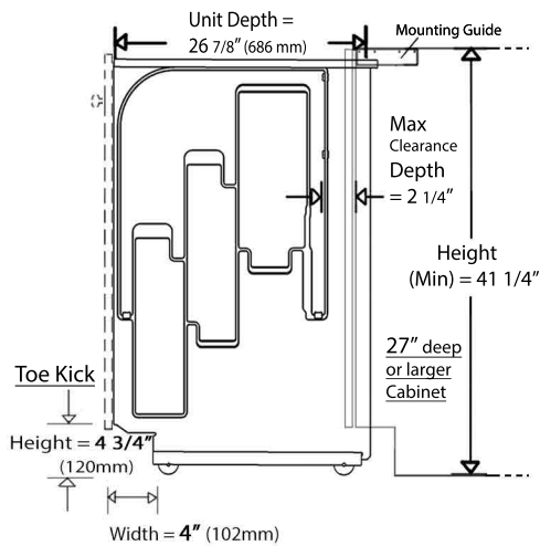
SIDE VIEW - Extended Closed Position (27" Model)
